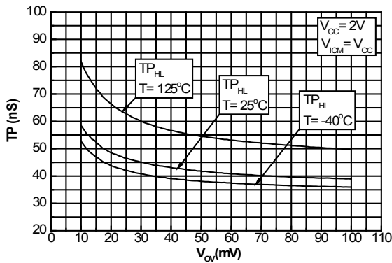
Figure 15. Propagation delay (HL) vs. overdrive at V_{cc} = 2V , V_{ictm} = V_{cc}
