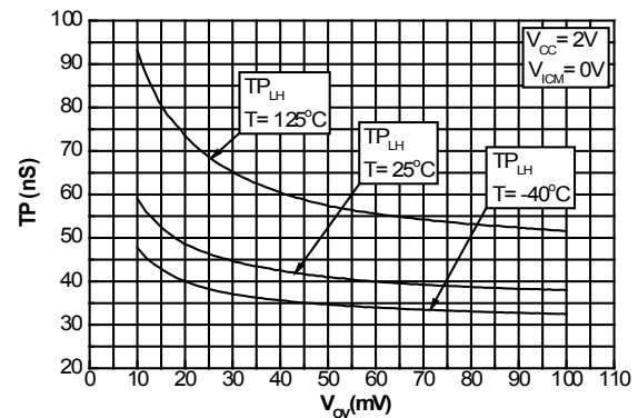
Figure 16. Propagation delay (LH) vs. overdrive at V_{cc} = 2V , V_{ictm} = 0V
