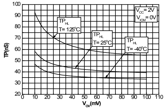
Figure 14. Propagation delay (HL) vs. overdrive at V_{cc} = 2V , V_{ictm} = 0V
