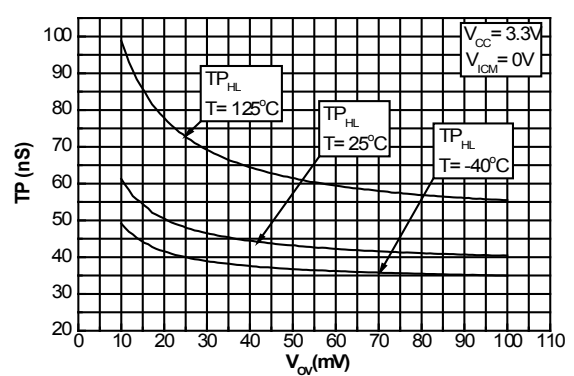
Figure 18. Propagation delay (HL) vs. overdrive at V_{cc} = 3.3V , V_{ictm} = 0V
